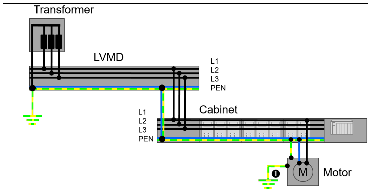
Figure 4.7: TN-C system with several connections to the equipotential bonding system
