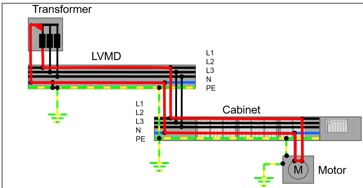
Figure 4.15: TN-S system with load and current flow
