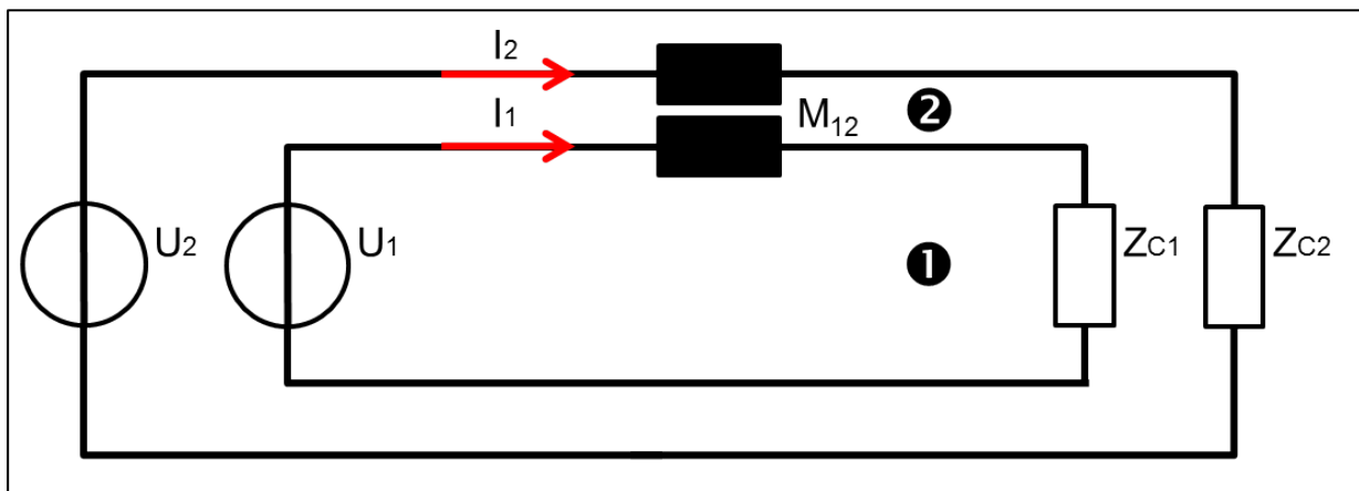
Figure 2.8: Inductive coupling
