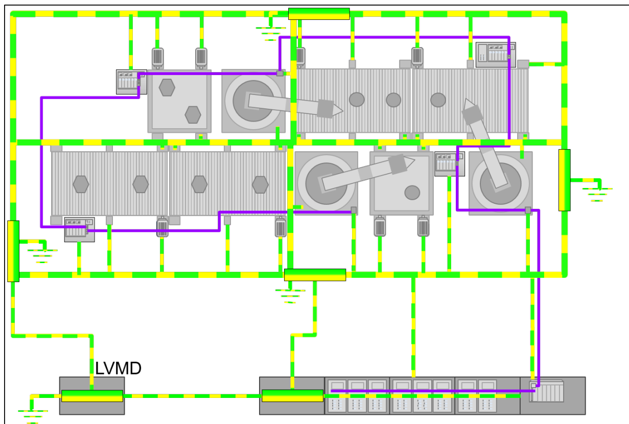
Figure 4.30: Meshed equipotential bonding
