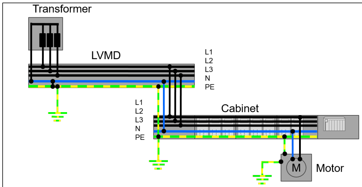
Figure 4.14: TN-S system with load
