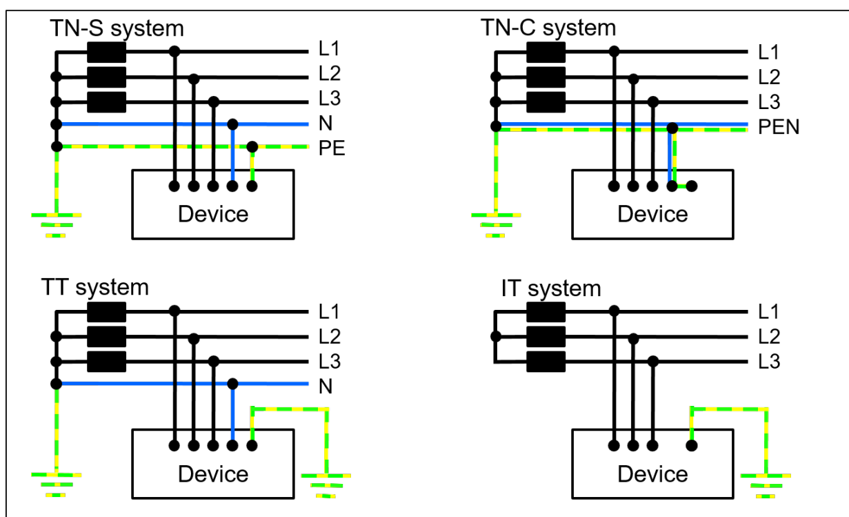
Figure 4.2: Network systems
