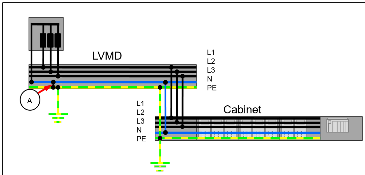
Figure 4.18: Ideal TN-S system
