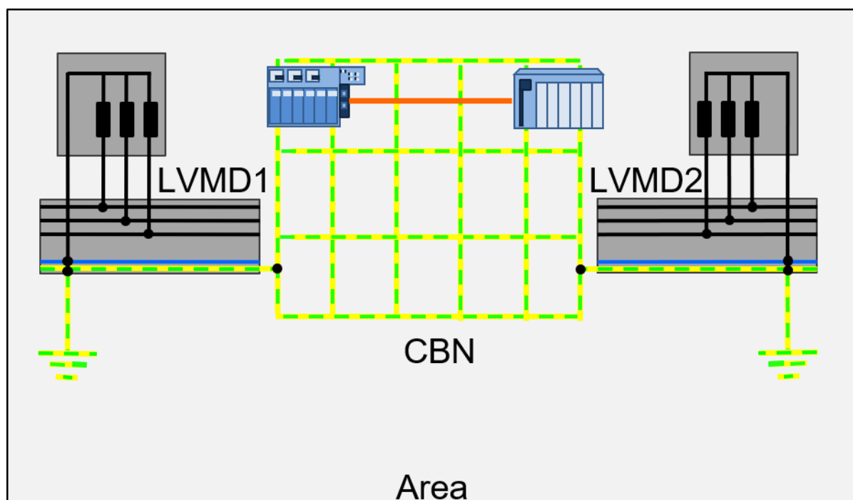
Figure 5.4: Continuous meshed CBN between plant sections
