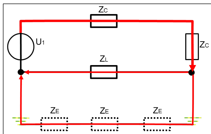
Figure 2.5: Conductive coupling in equipotential bonding system 3
