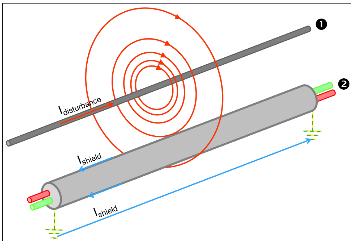
Figure 3.3: Induction in the cable shield
