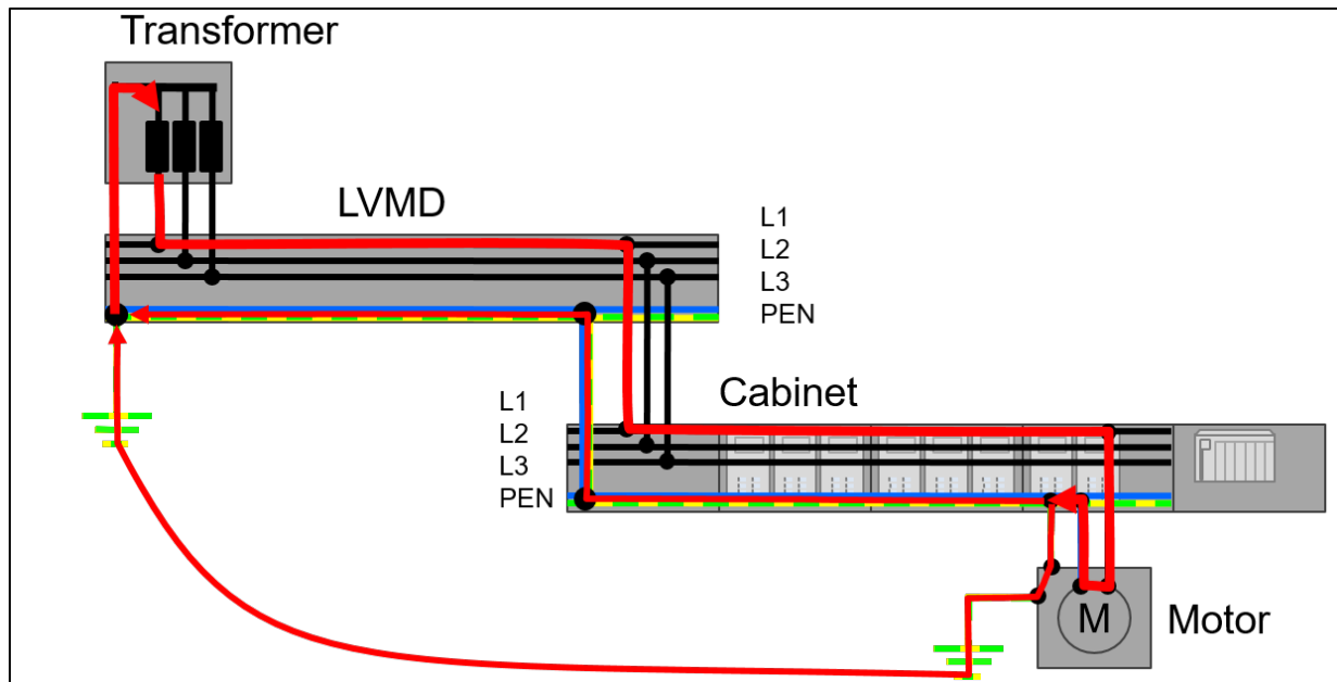
Figure 4.8: TN-C system with multiple earthing, load and current flow
