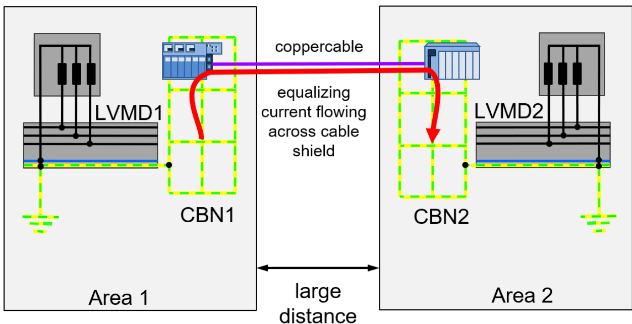
Figure 5.2: Copper cable between plant sections
