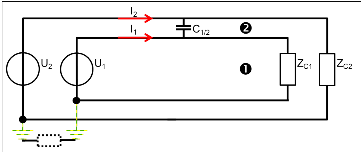
Figure 2.7: Capacitive coupling
