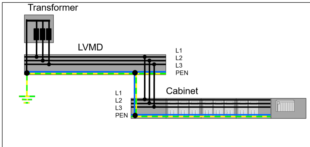
Figure 4.4: TN-C system
